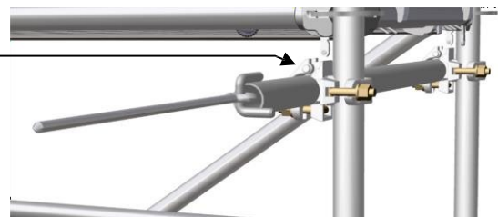
Collier orthogonal (SWS-19-9902)
